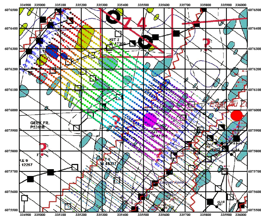
Figure 62- Grid Extension with geology underlay
