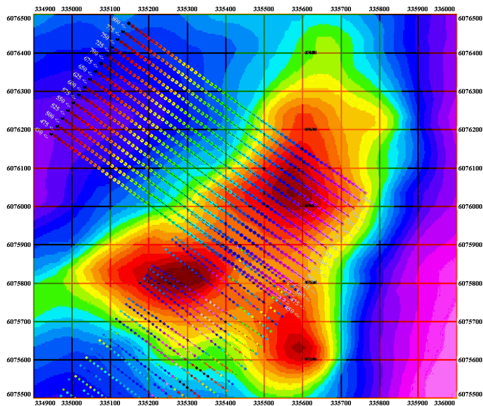
Figure 60 – Grid Extension with aeromagnetic total field underlain
