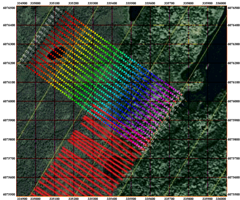
Figure 59 – Grid Extension with 2018 grid in red
