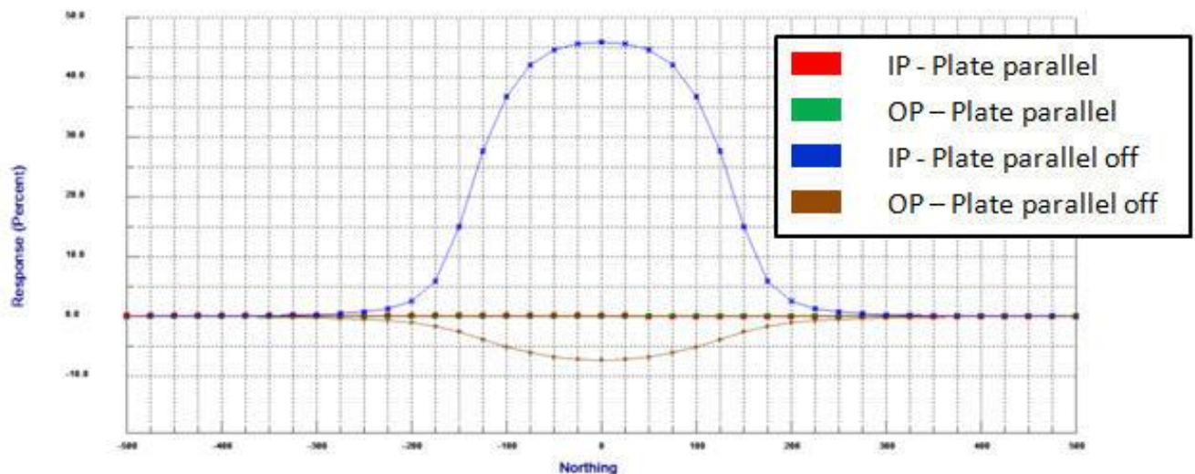
Figure A4: NS strike, NS polarization
