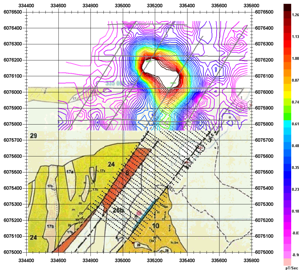
Figure 49 – VTEM Ch24 (2.3msec)
