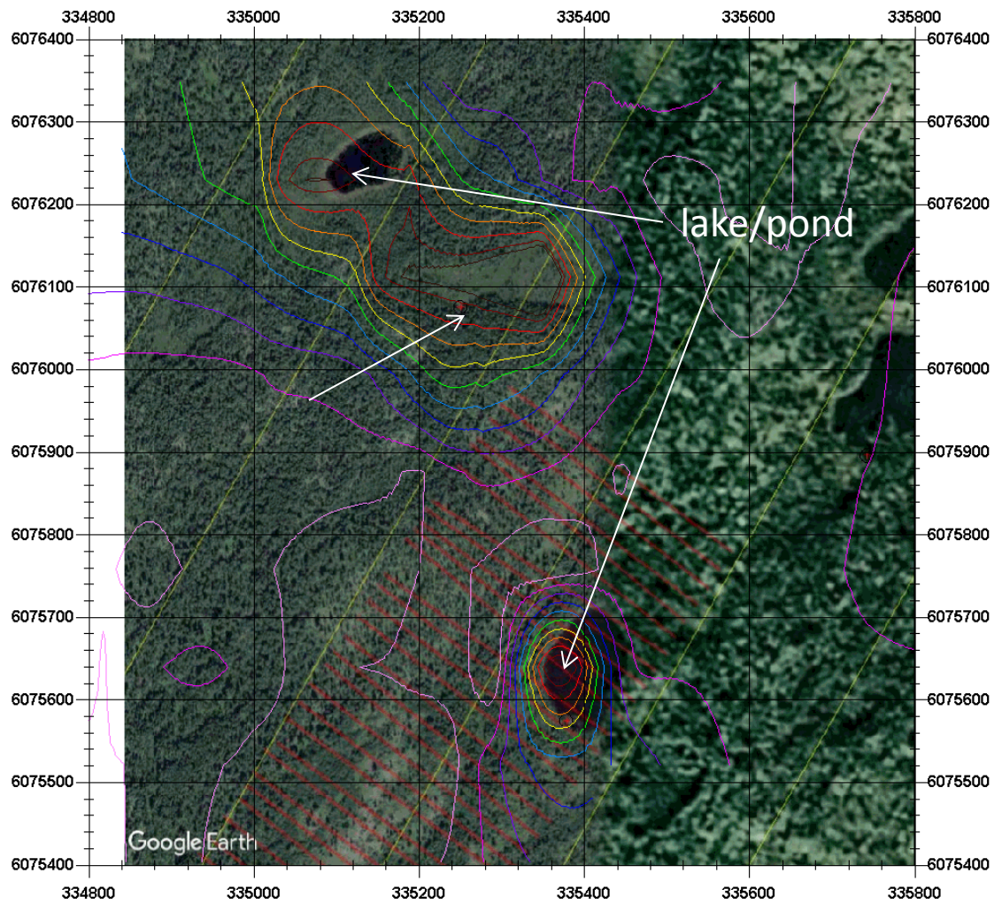
Figure 45 – Ground features as illuminated by the early time VTEM
