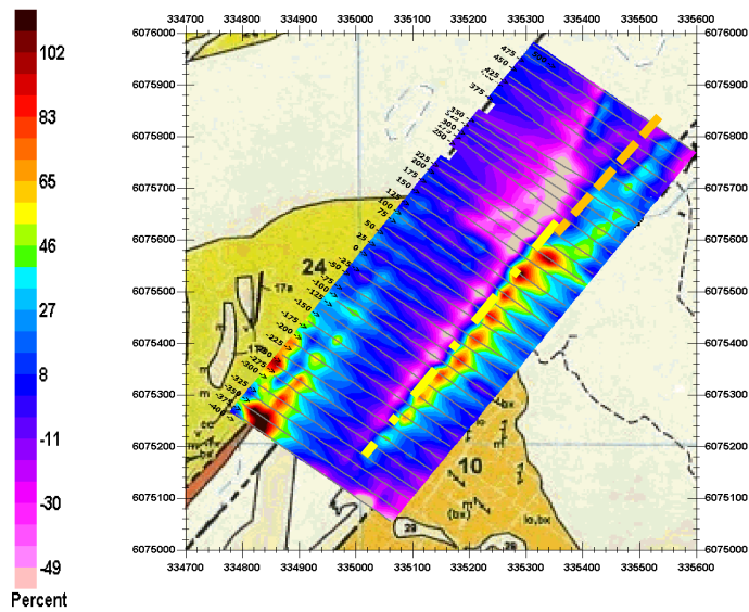
Figure 27 InPhase Hz (IP) Seattle contoured Geology map underlain
