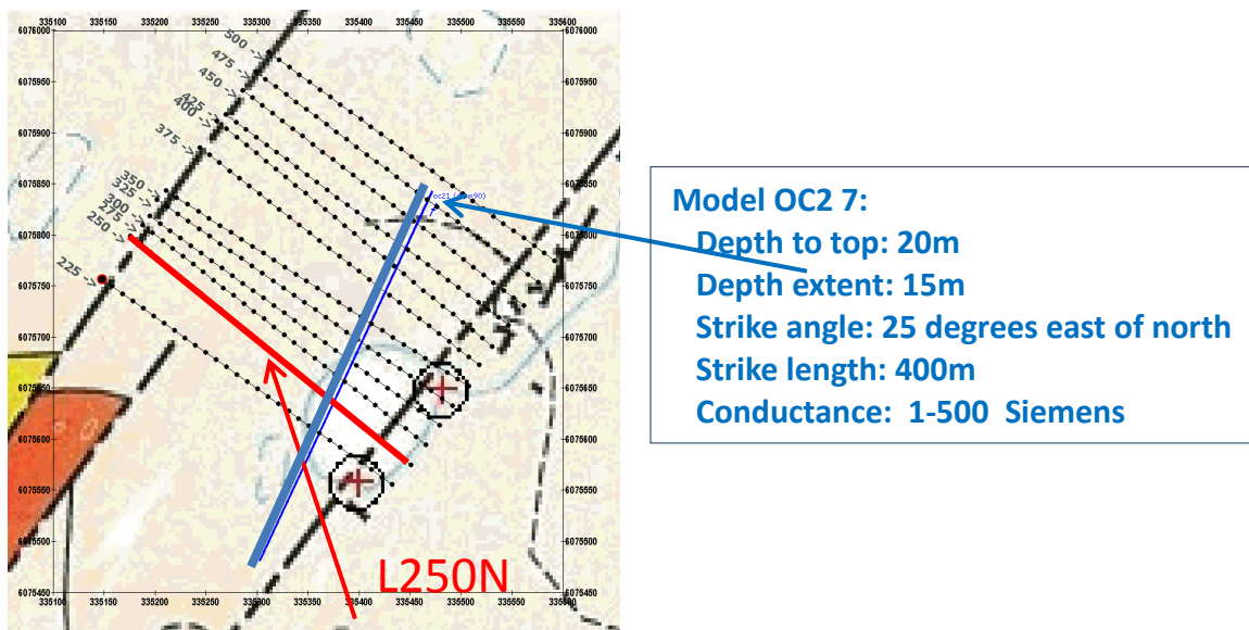
Figure 41a –C02 – Line 250N) with model OC2-7
