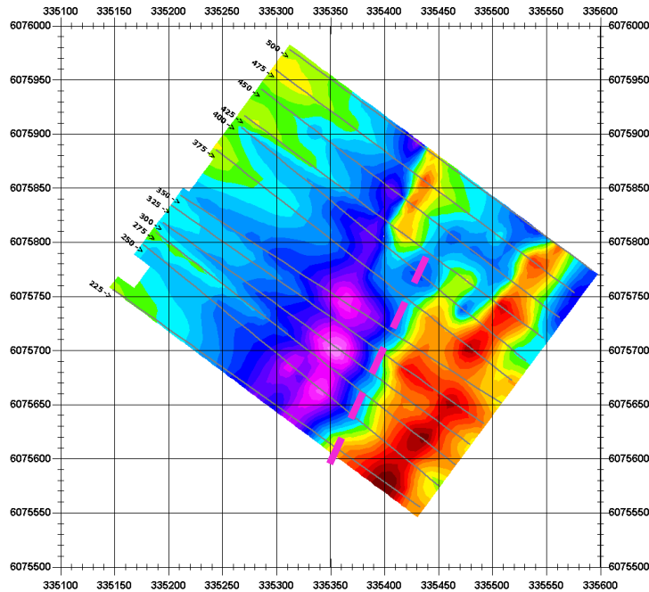
Figure 36 – InPhase (IP) Seattle across C02– L225-500N
