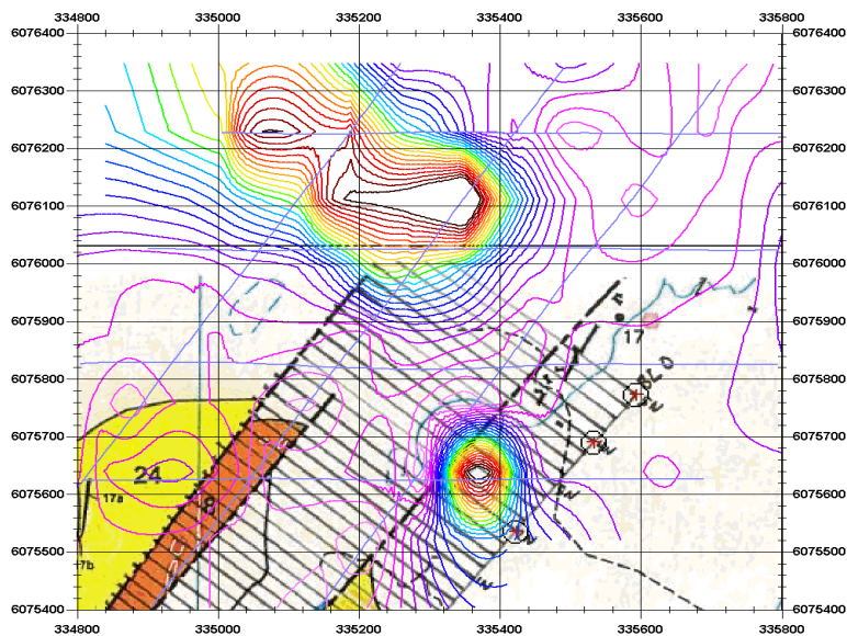
Figure 47– VTEM Ch5 with VLF grid and geology underlain
