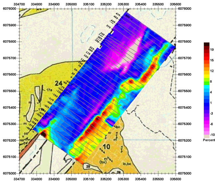
Figure 28 Out of Phase Hz (OP) Seattle contoured
