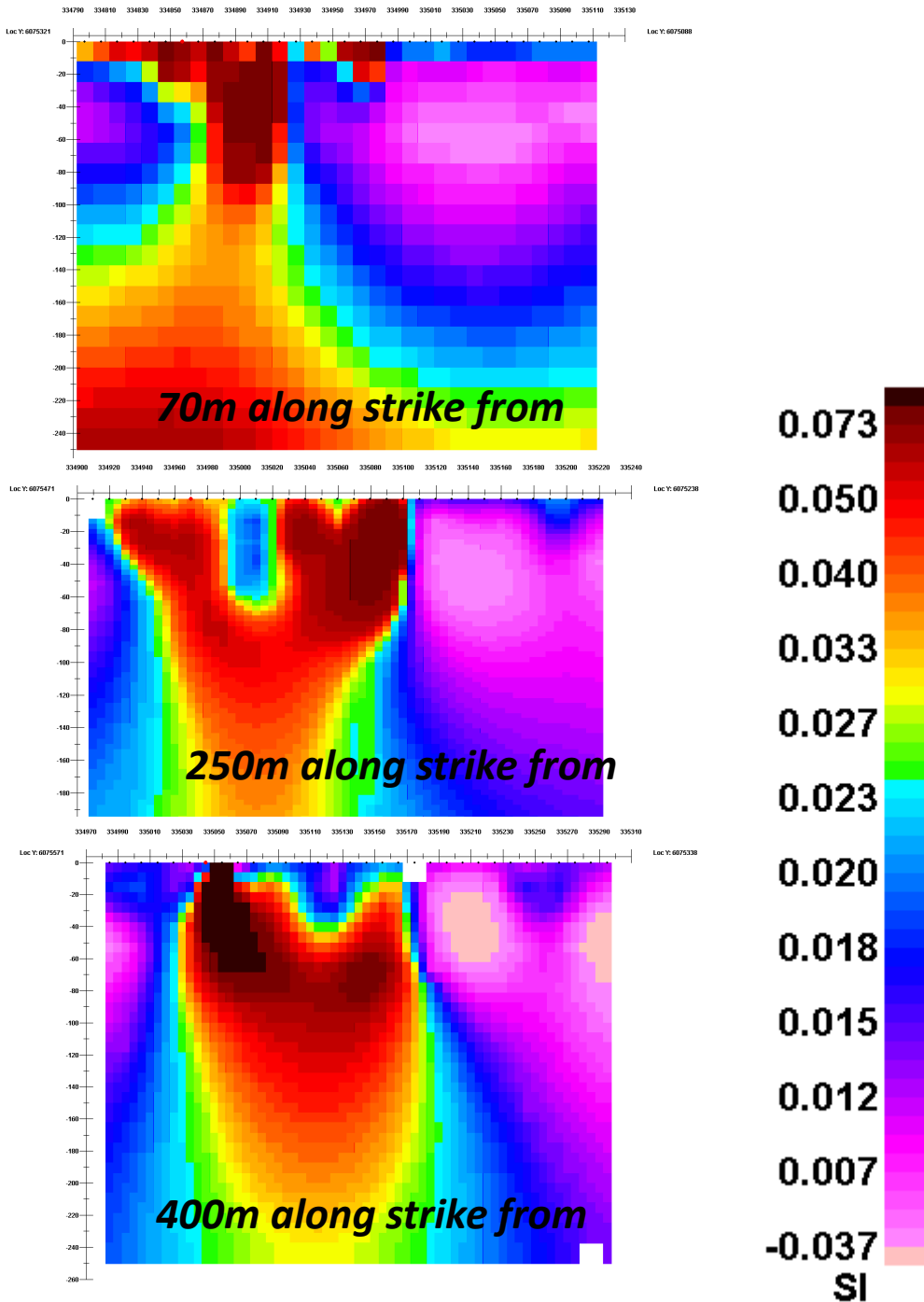
Figure 14: Inversion sections perpendicular to strike southern end
