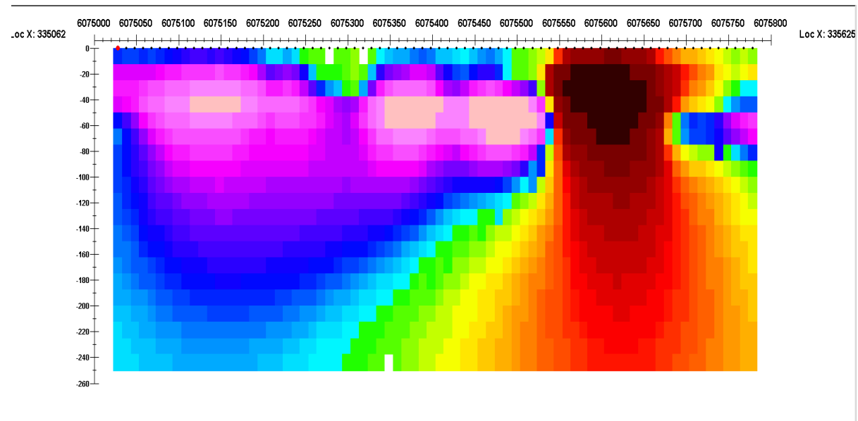
Figure 11: Inversion section parallel to strike (37 degrees east of north)
