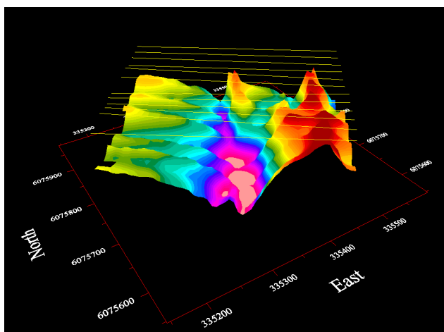
Figure 37– The IP response represented as a surface.
