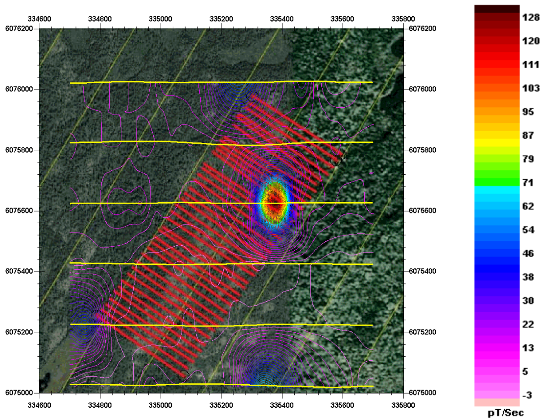
Figure 43 – VTEM early time with satellite underlay
