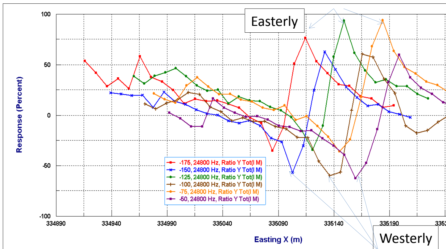
Figure 29 –Response shift IP Seattle across C91 – 6 lines
