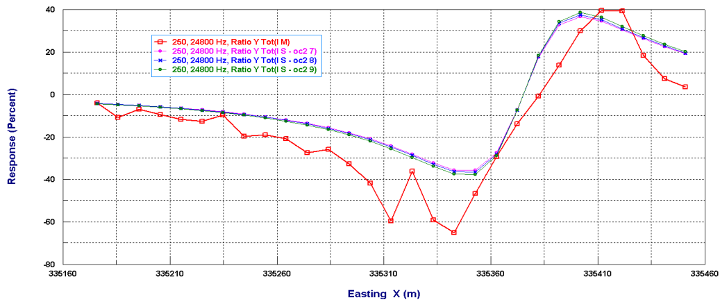
Figure 41b – InPhase (IP) Seattle across C02 – Line 250SN
