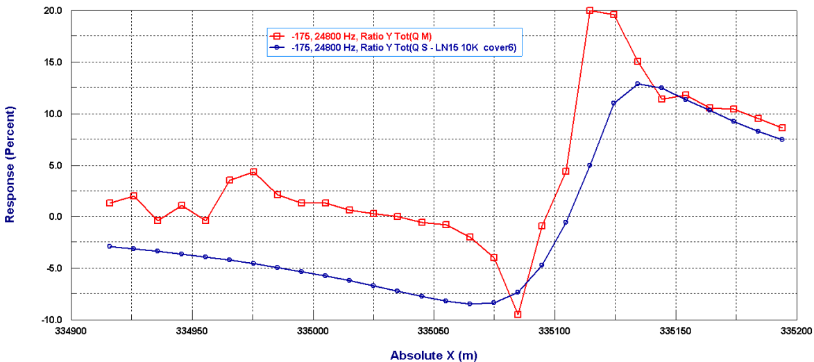
Figure 35 – Out of Phase (IP) Seattle across C01 – Line 175S – data plus model
