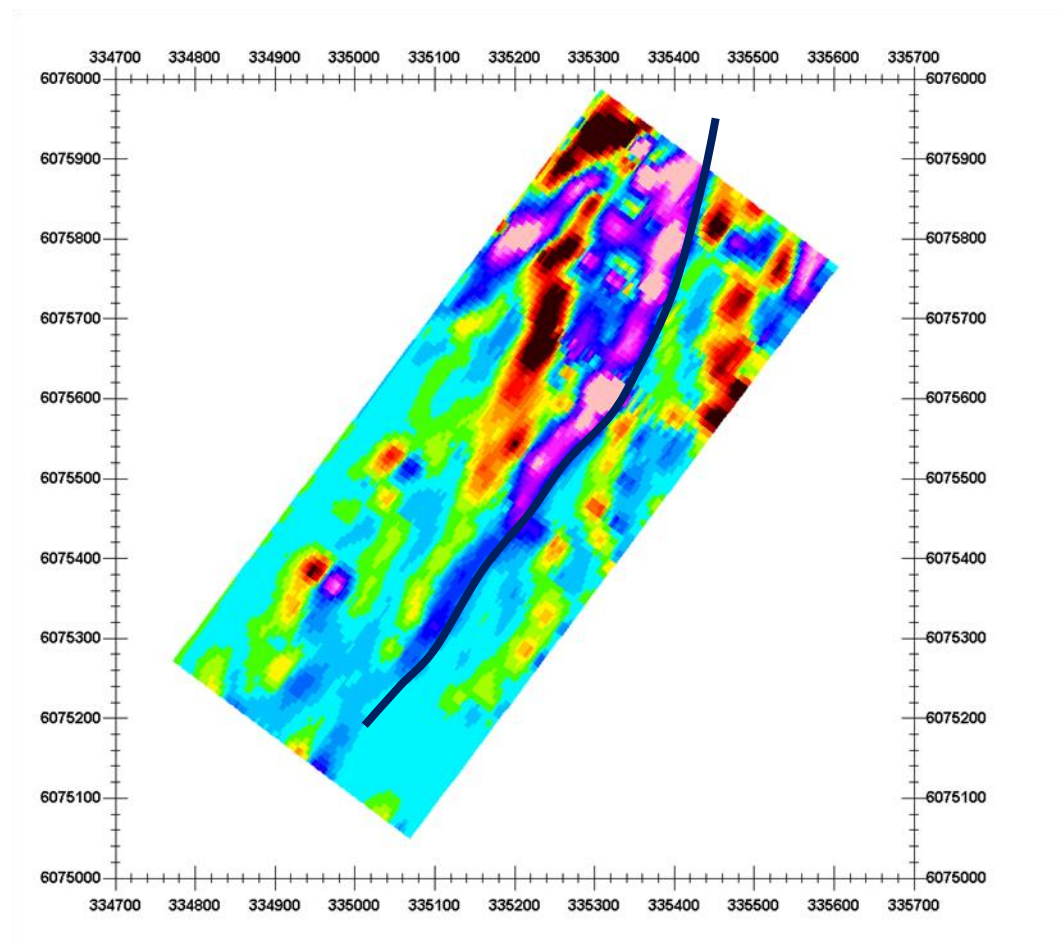
Figure 58– Ground magnetics Horizontal derivative along profiles
