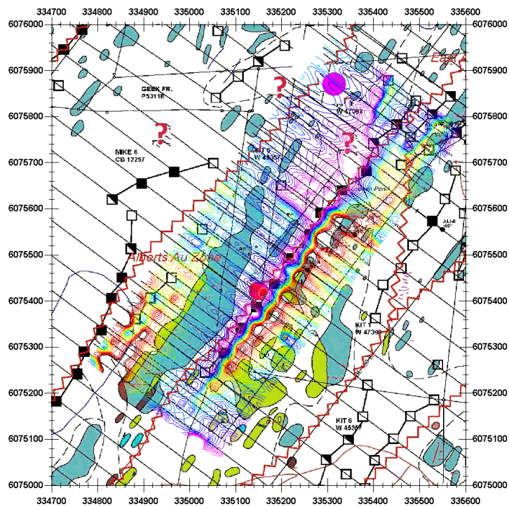
Figure 26 InPhase Hz (IP) Cutler with Geology underlay
