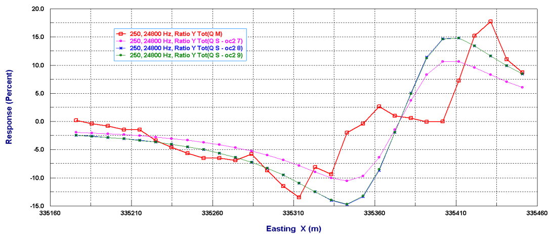
Figure 42 – Out of Phase (OP) Seattle across C02 – Line 250N
