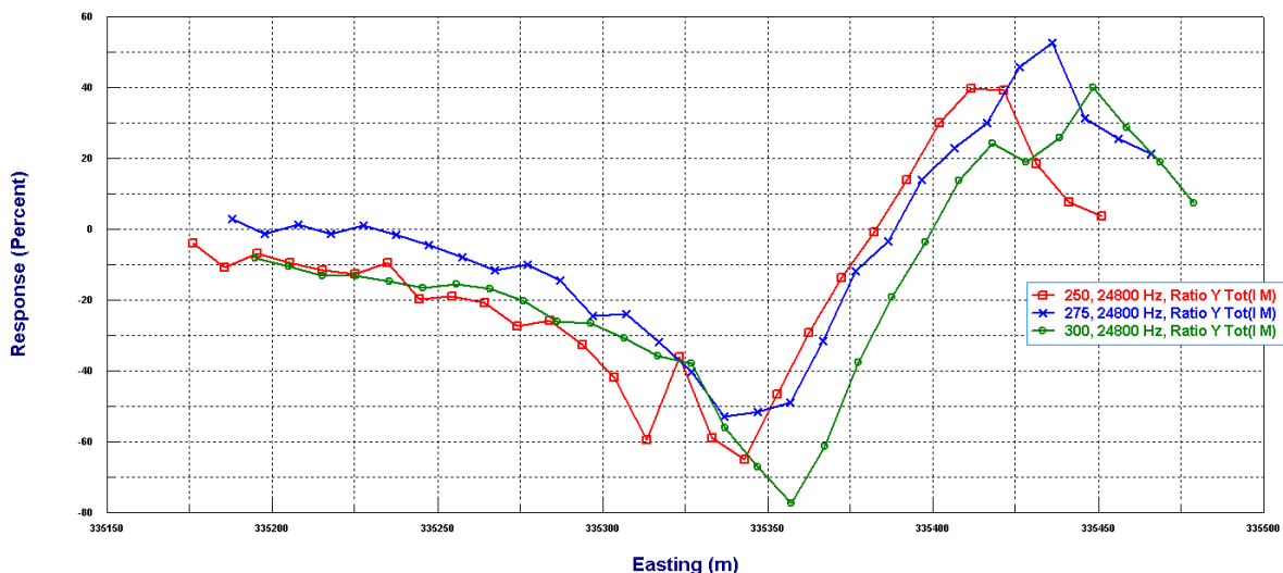
Figure 38 – InPhase (IP) Seattle across C02 L250-L300
