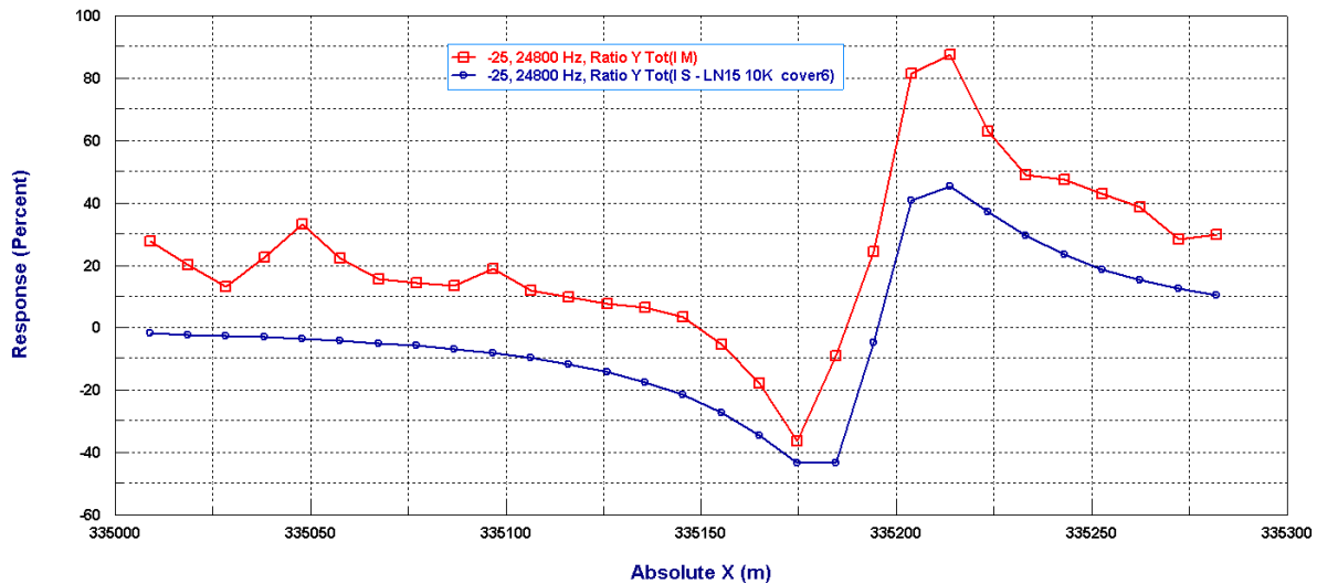
Figure 34 – InPhase Hz (IP) Seattle across C01 – Line 25S – data plus model
