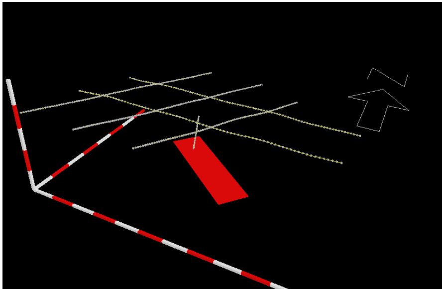
Figure 53 - NW Anomaly 3D view with VTEM lines and borehole
