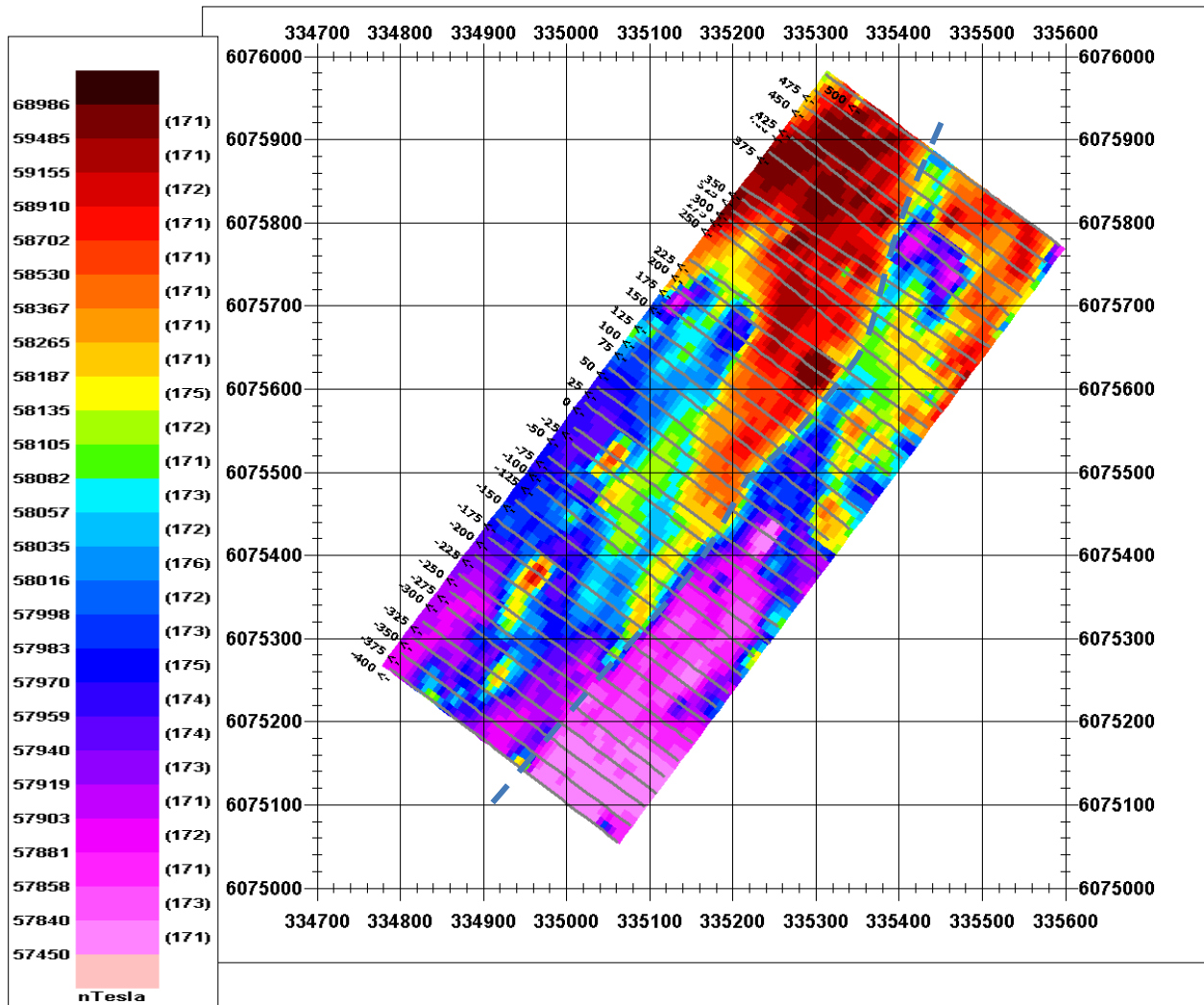
Figure 6: Equal weight magnetic data with structural boundary
