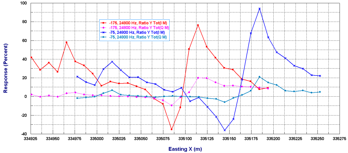
Figure 30 – InPhase/Out-of-Phase Hz (IP/OP) Seattle across C01 – 2lines (-175,-75)
