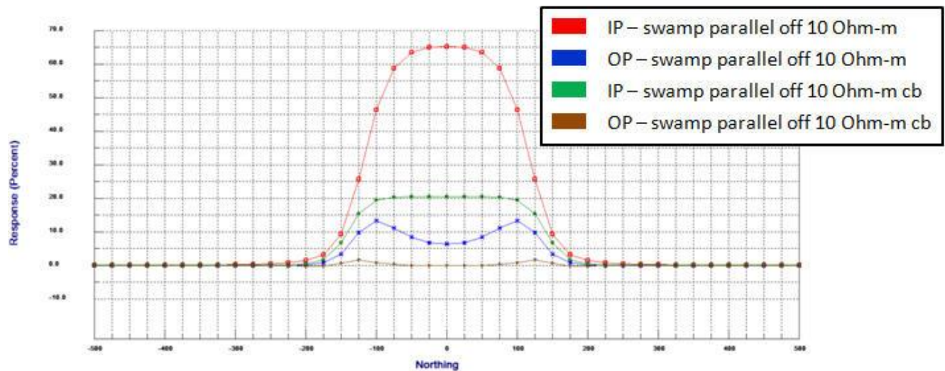
Figure A5: NS swamp, NS polarization of source
