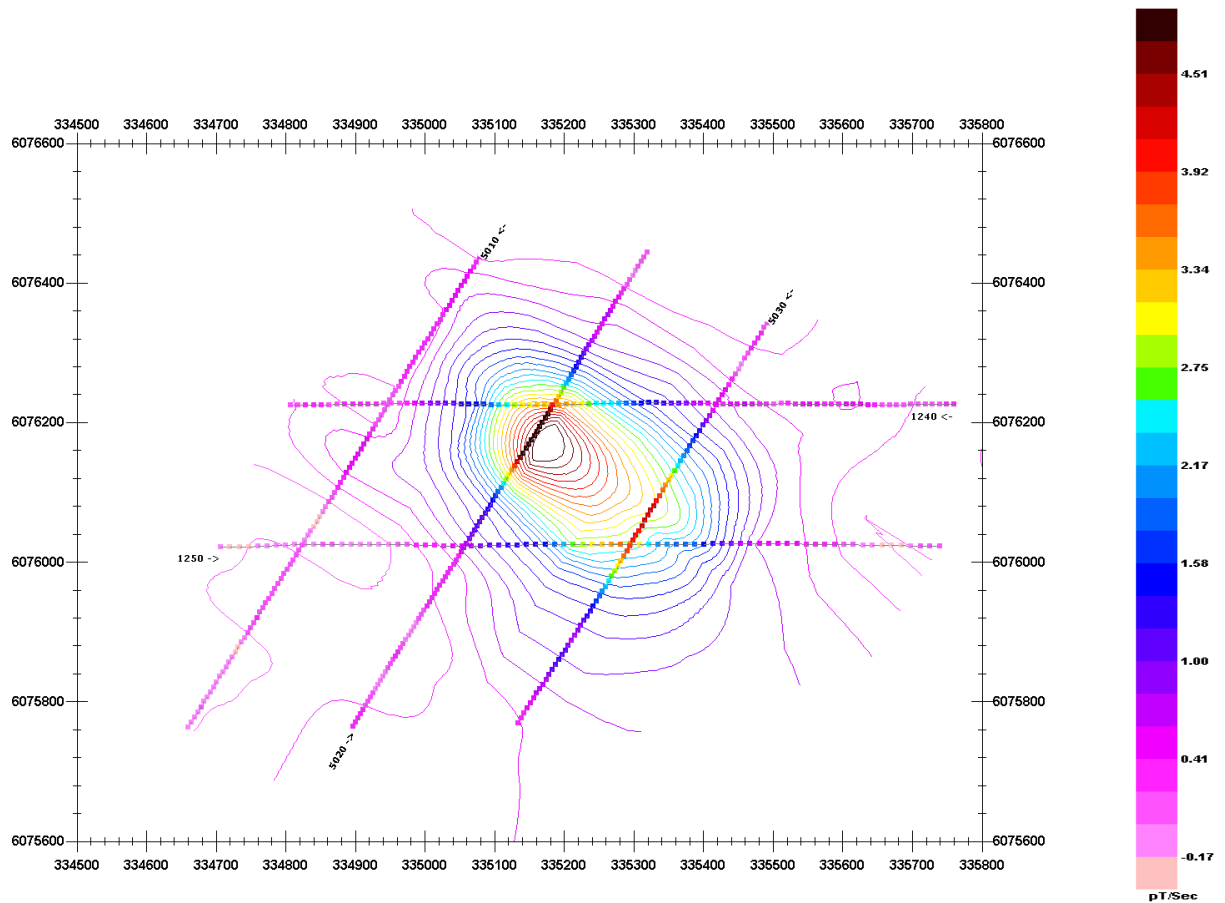
Figure 50 – VTEM Ch18 contours and actual point data
