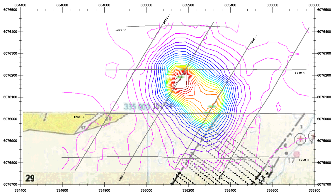
Figure 48– VTEM Ch16
