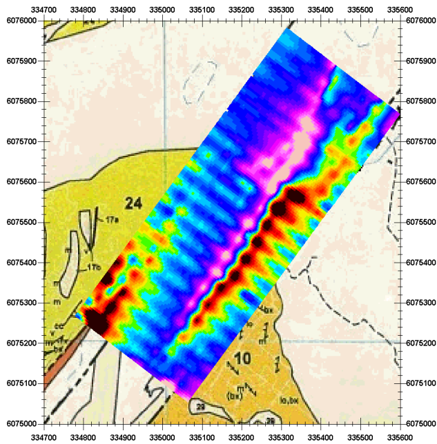
Figure 55 – VLF Seattle In-Phase
