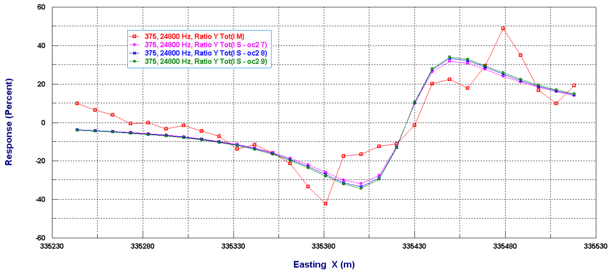
Figure 40 – InPhase Hz (IP) Seattle across CO2, L375
