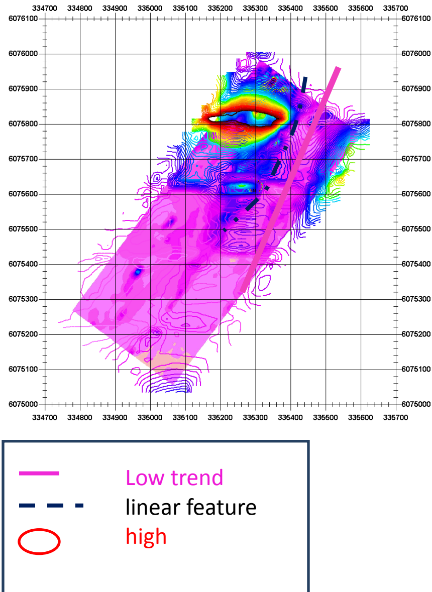
Figure 22: Aeromagnetic data analytic signal contoured with ground mag underlain
