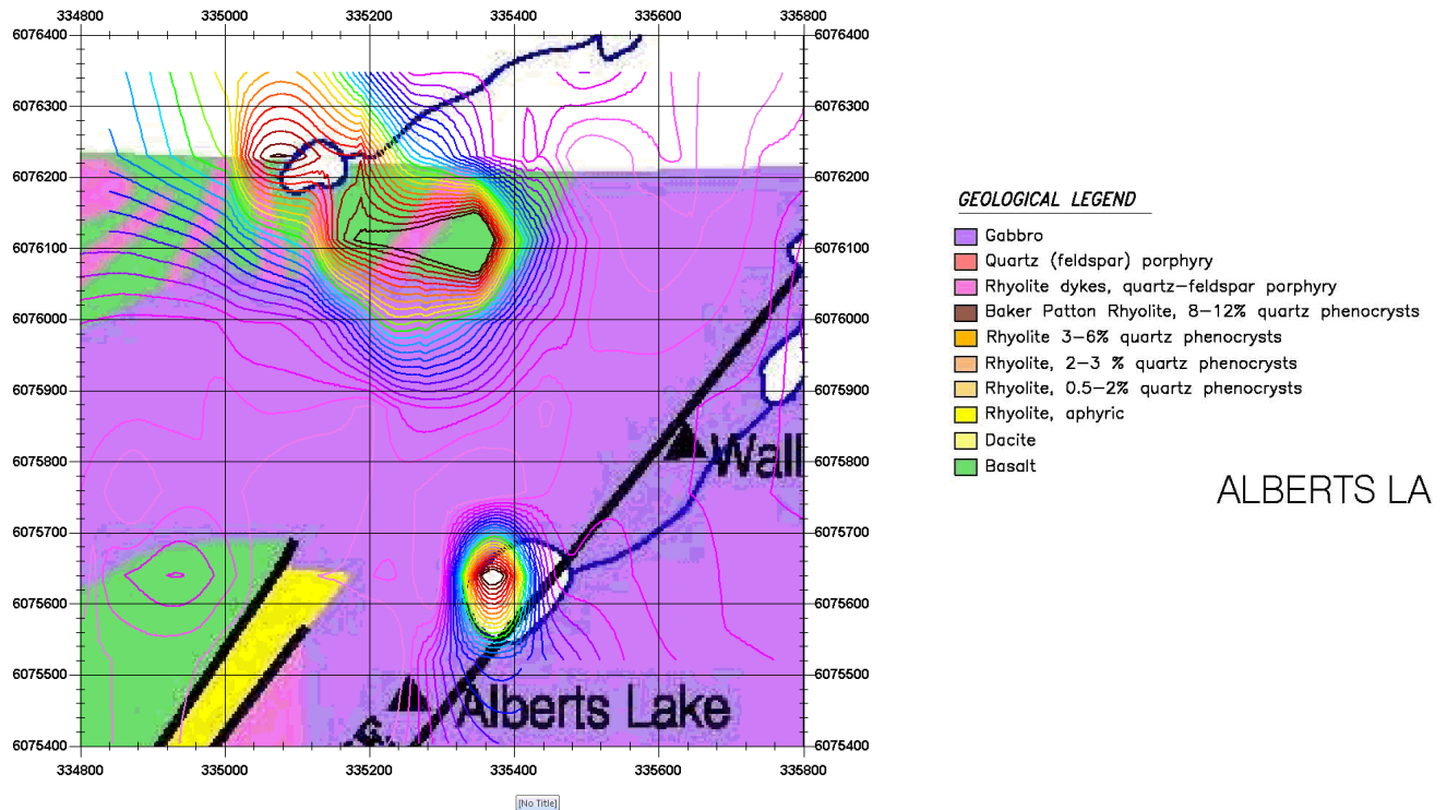
Figure 46 – VTEM Ch5 vs Geology
